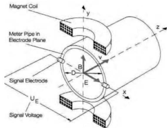
Electromagnetic flow meter schematic
